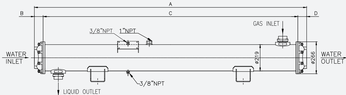
COUNTERCURRENT CONDENSER
